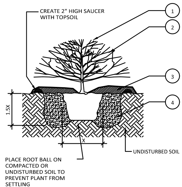
CONTAINER SHRUB PLANTING DETAIL LD 02 N.T.S.
