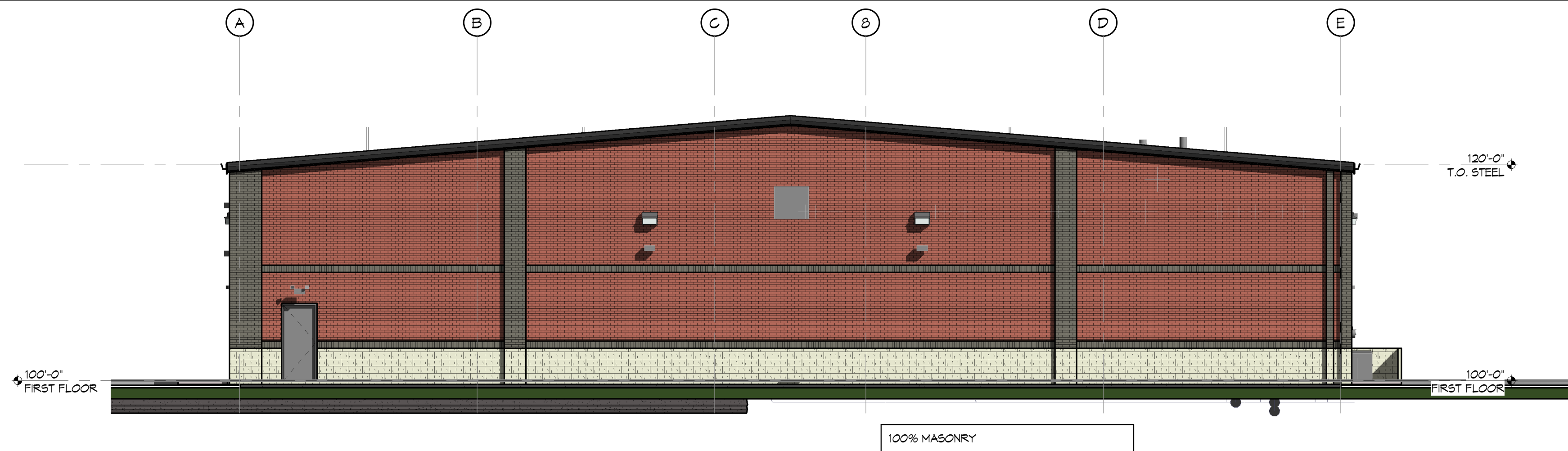
4 WEST ELEVATION COLOR 1/8" = 1'-0"
