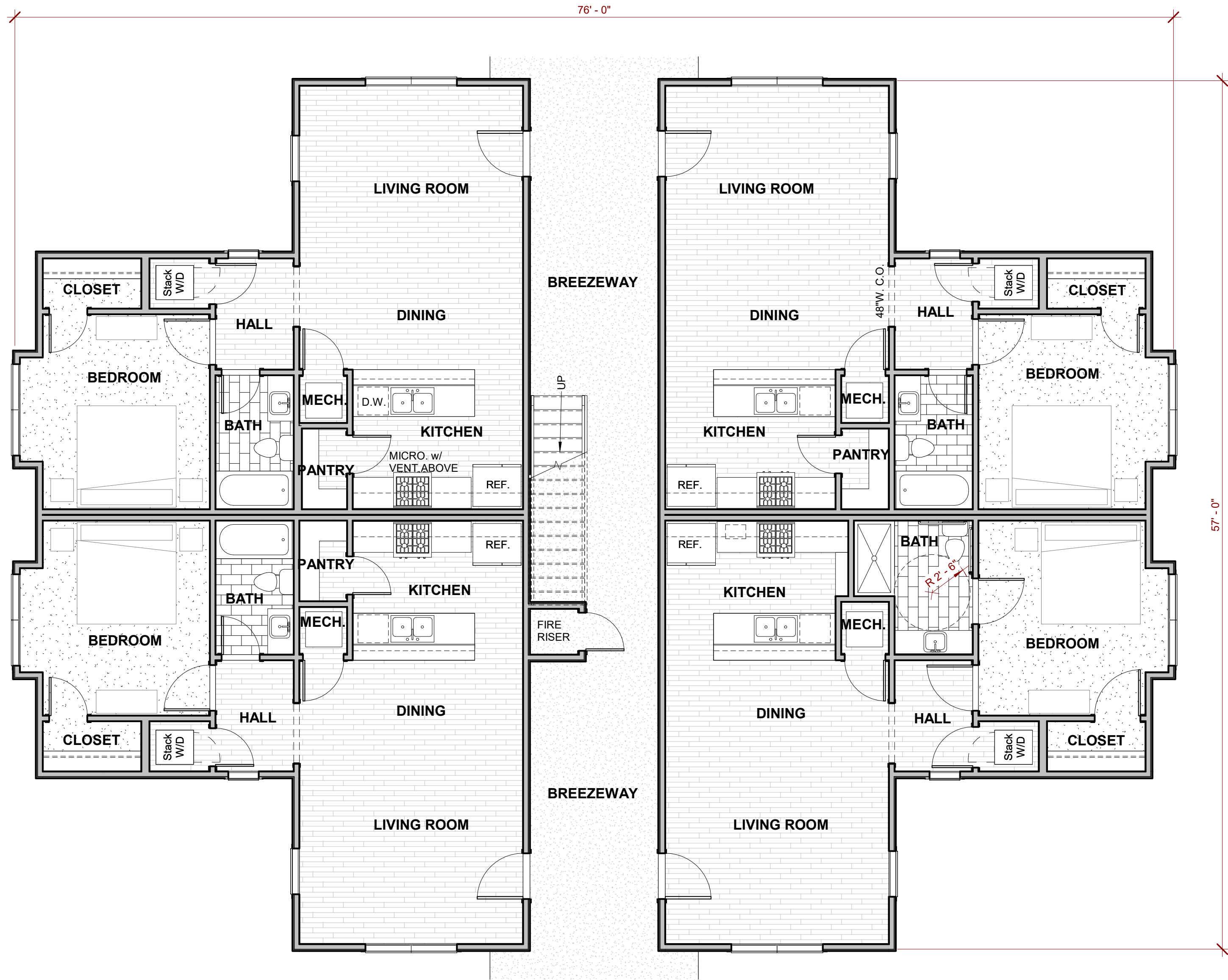
4 FIRST FLOOR PLAN. 3/16" = 1'-0"
