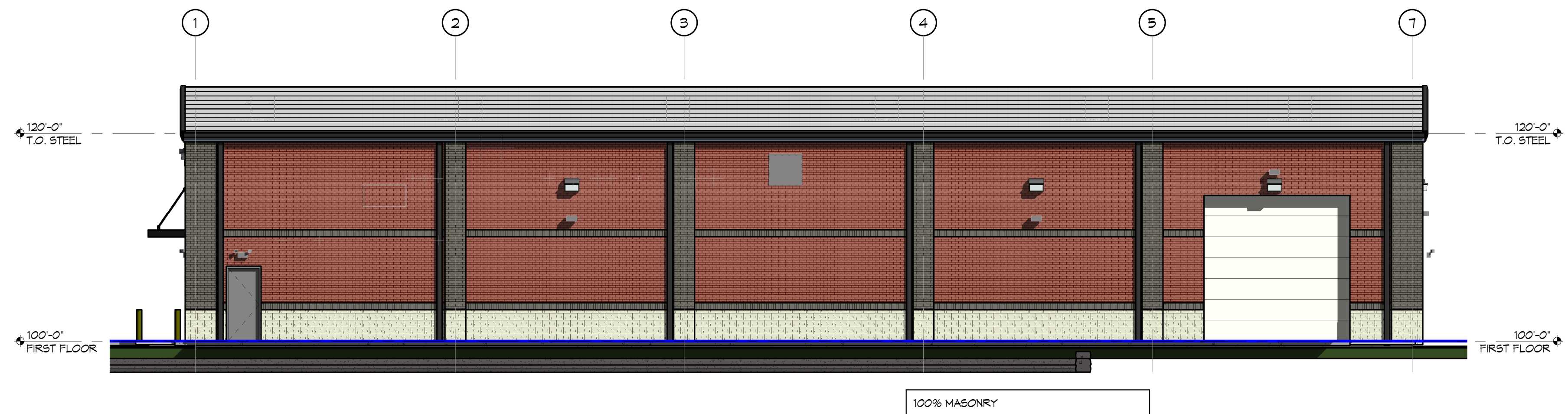
2 NORTH ELEVATION COLOR 1/8" = 1'-0"
