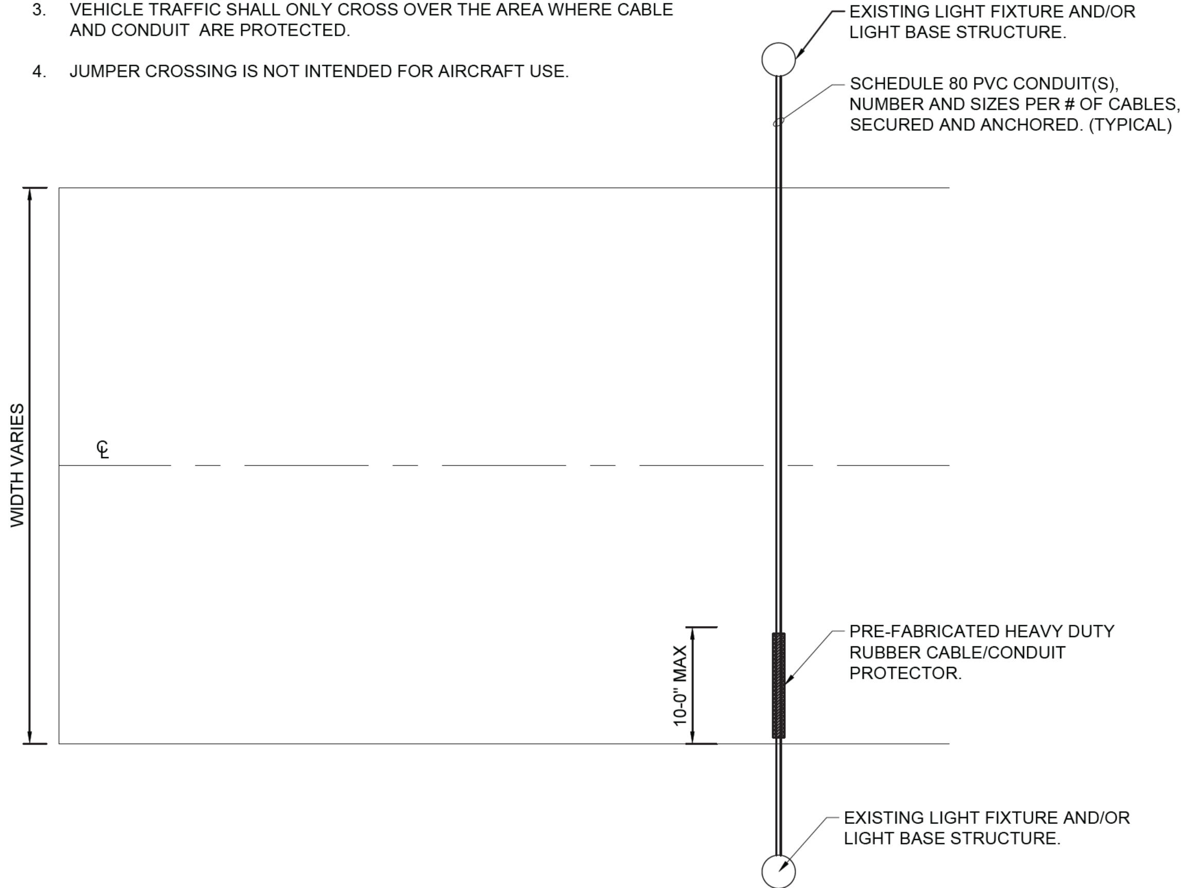
1 GC-203 TYPICAL PAVEMENT JUMPER CROSSING FOR TEMPORARY AIRFIELD LIGHTING SCALE: NONE
