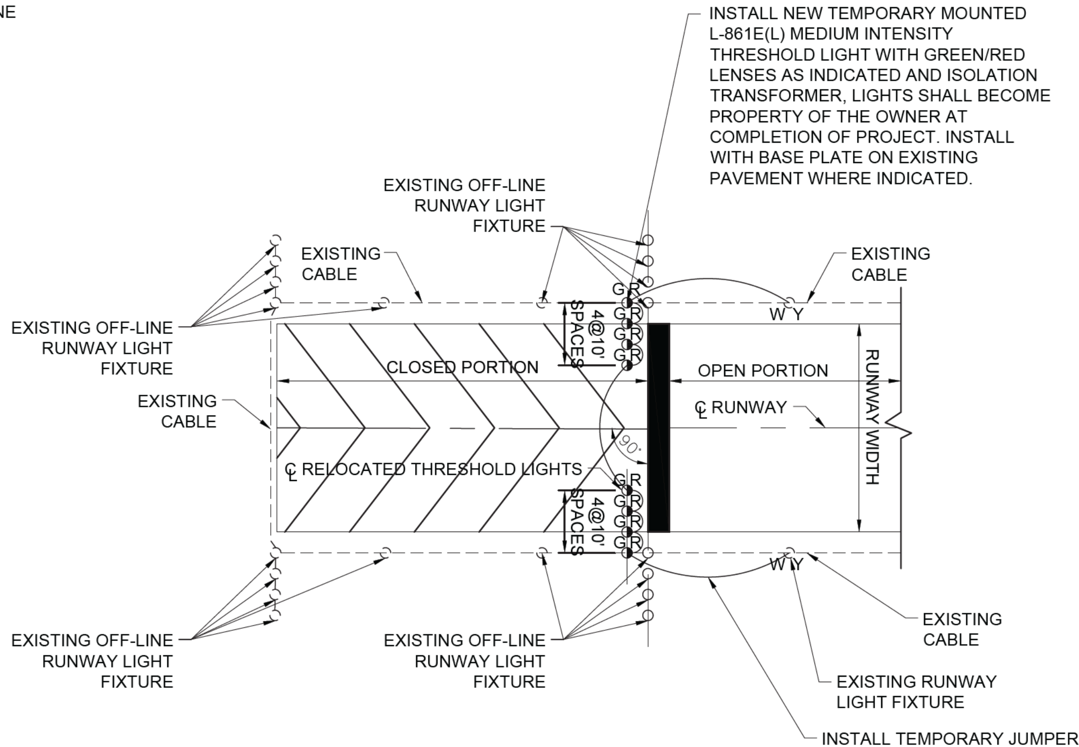
2 GC-203 TEMPORARY DISPLACED THRESHOLD SCALE: NONE
