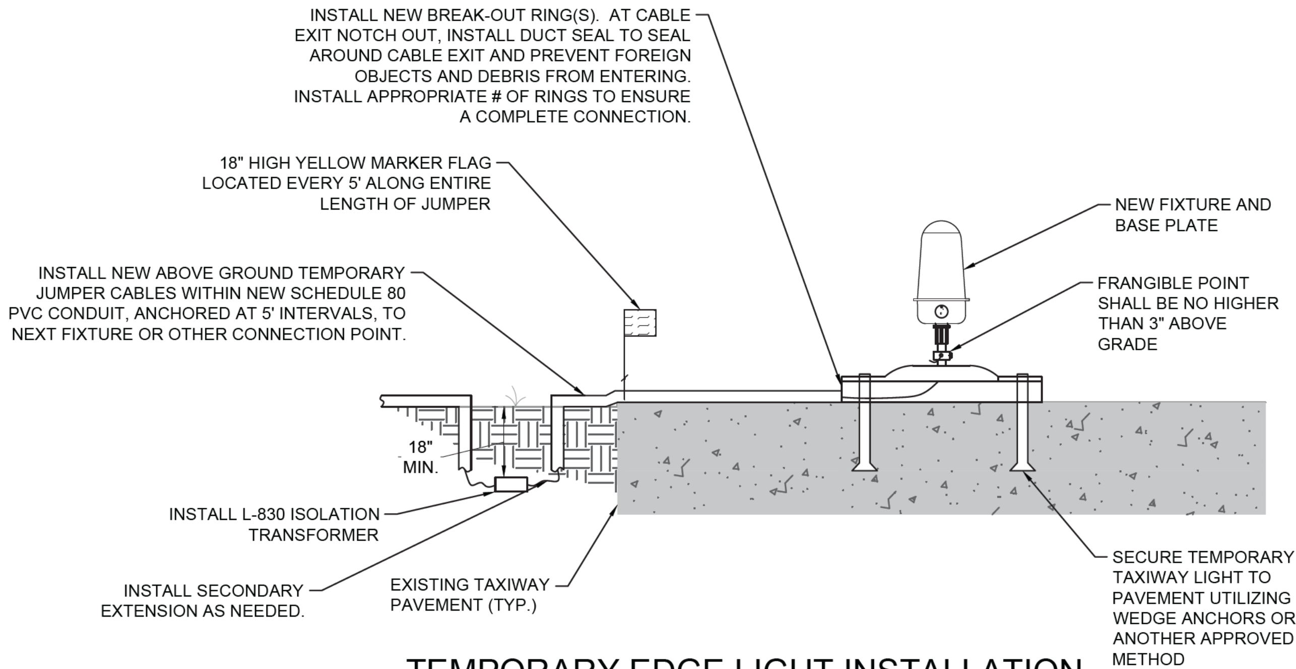
3 GC-203 TEMPORARY EDGE LIGHT INSTALLATION ON EXISTING PAVEMENT SCALE: NONE
